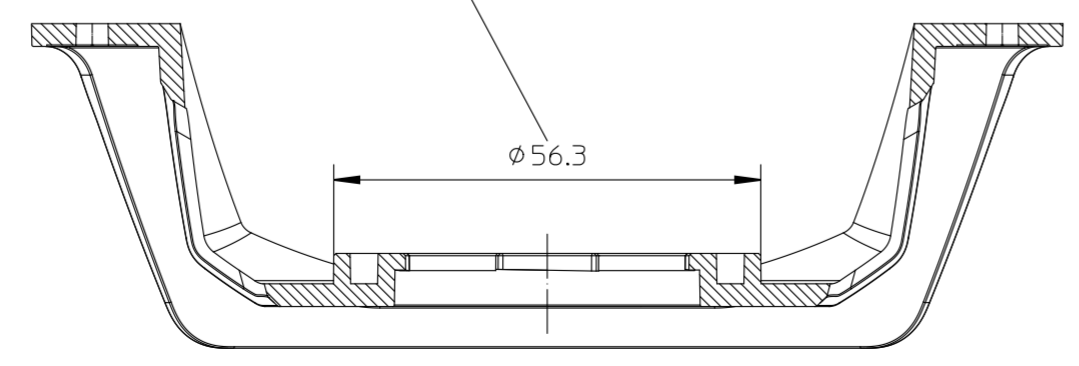
Section Y-Y
